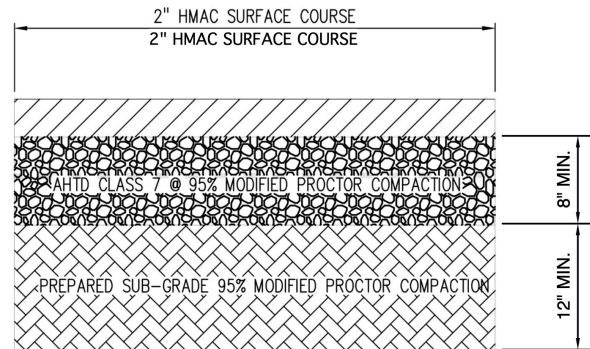
TYP. ASPHALT PAVING SECTION N.T.S.
